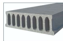
Hollow-core slab
